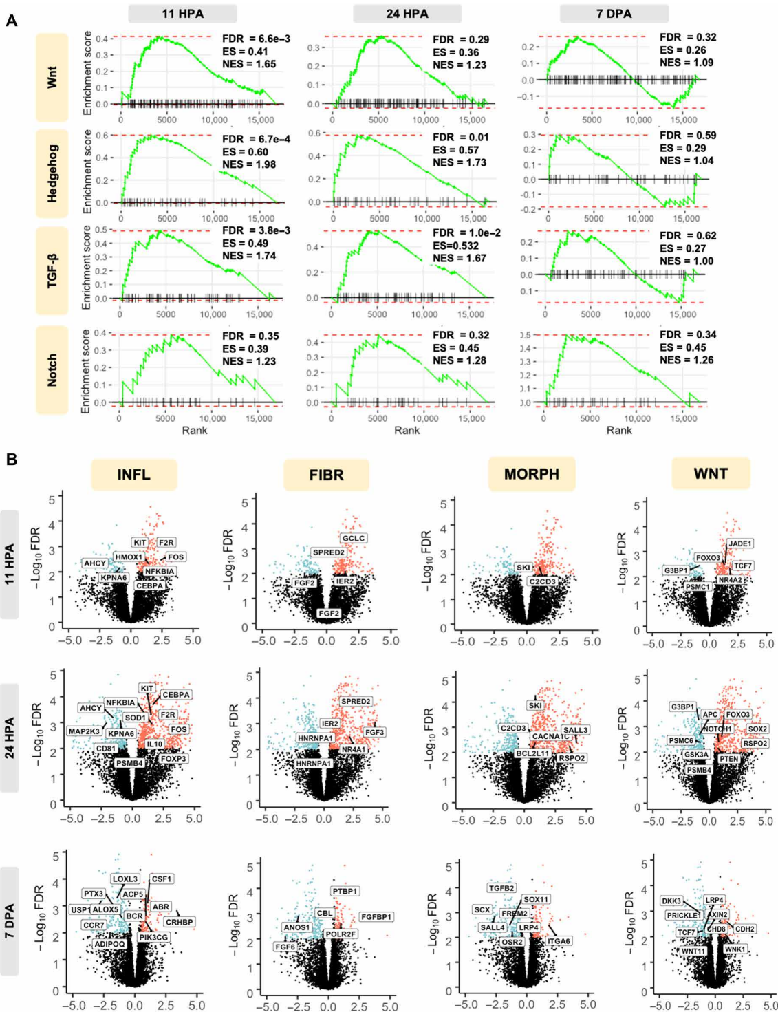
Fig. 4. Transcriptomic changes reflect regeneration-focused signaling mechanisms. (A) GSEA enrichment plots displayed major signaling pathways involved in cell morphogenesis that were up-regulated in the early blastema in MDT-exposed animals relative to ND. Specifically, up-regulated genes enriched within each KEGG term are shown within each GSEA plot. FDR (adjusted P value), enrichment score (ES), and normalized ES (NES) are presented with each plot. Cell morphogenesis-related signaling peaks at 11 hours and decreases over time, with WNT, hedgehog, and TGF- \beta displaying no significant differences in differential gene expression between MDT and ND 7 dpa. (B) Volcano plots depict statistical significance (FDR; adjusted P value) versus magnitude of change (fold change) for rapid visual identification of genes. Data points, representing individual genes, highlight fold change values that are also statistically significant. Statistical significance is measured by -\log_{10}(\text{FDR}) . The fold change was measured by \log_{2}(\text{FC}) [cutoff at \log_{2}(\text{FC}) > 0.05 ]. Significant GO pathways comparing MDT and ND groups 11 hours, 24 hours, and 7 days comparing MDT versus ND are displayed. Biologically significant results include KIT and IL10 for inflammation (INFL), FGF for fibroblast (FIBR), which varies as a function of time, and SALL4 for appendage morphogenesis (MORPH), which is up-regulated and typically observed during scar-free wound healing in axolotls.
